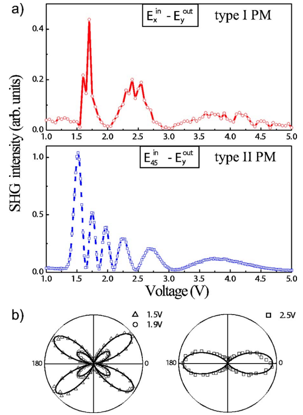
FIG. 2. (Color online) (a) SHG intensity as a function of the applied voltage amplitude for E_x^{\text{in}}E_y^{\text{out}} and E_{45}^{\text{in}}E_y^{\text{out}} polarization combinations; (b) the SHG rotational anisotropy patterns at different voltages for crossed polarization combinations. At 0^\circ the polarizer is pointing along the director and the analyzer perpendicular to it. Solid curves are fits by Eqs. (5) and (6).
